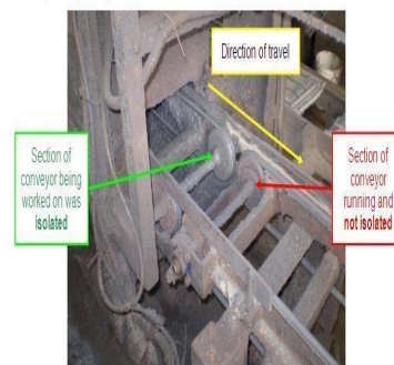
Conveyor
